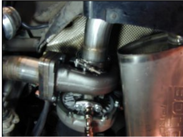
Photo 13.4. Muffler mounted on turbo with V-Band clamp.
