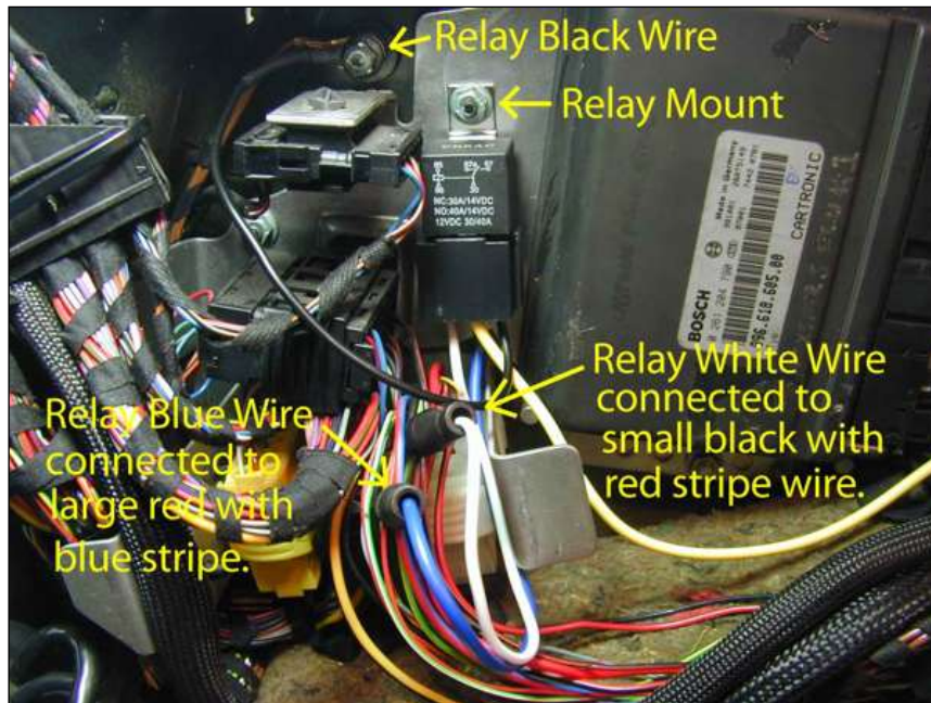
Photo 11.1. Relay connections.
